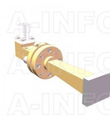
LB-15-10-C-1.85FSPO Standard Gain Horn Antenna 50-65GHz 10dB Gain 1.85mm Female
