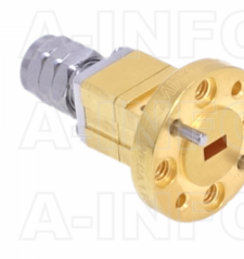
15WECA1.85M_Cu Endlaunch Rectangular Waveguide to Coaxial Adapter 50-65GHz WR15 to 1.85mm Male
